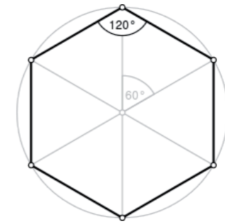
REGULAR HEXAGON
