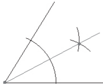
ANGLE BISECTOR
