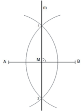
PERPENDICULAR BISECTOR
